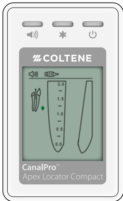
File tracking
